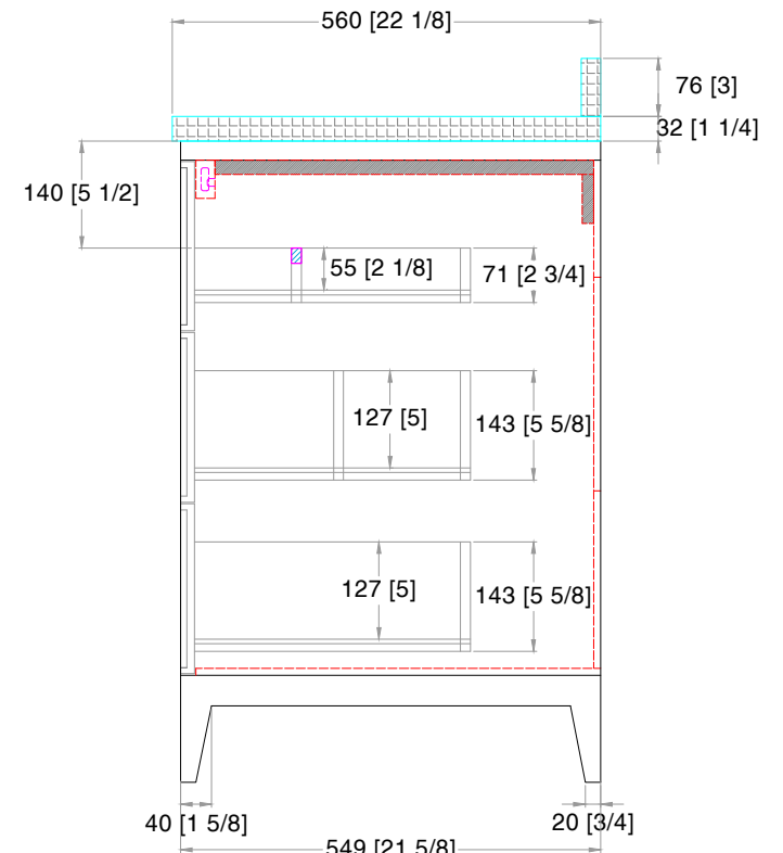
SIDE VIEW
